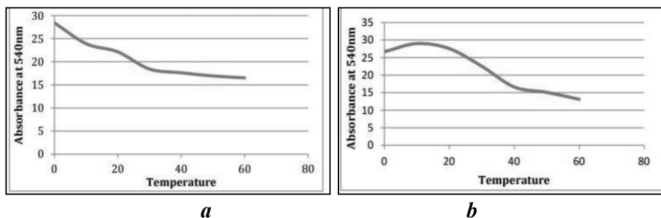
Figure 4. Stability of betacyanines at different temperatures in the dark(a), in the light (b)
