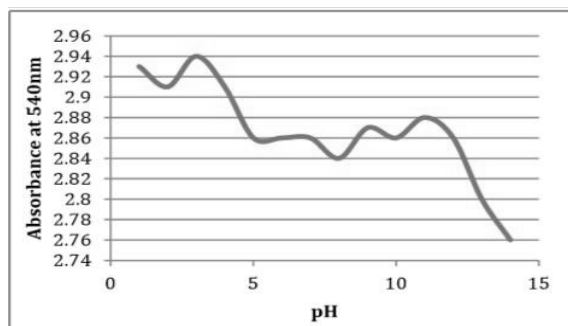
Figure 5. Stability of betacyanines at different pH
