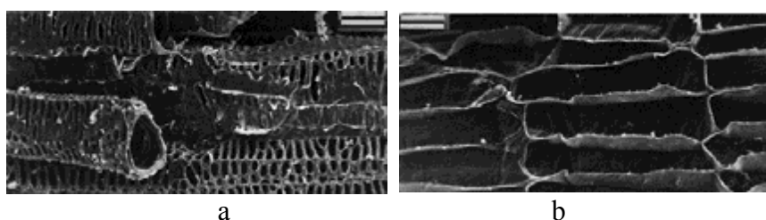
Figure 1. Scanning electron micrograph of a cross section of sugar beet: a) an incision of one of the vascular bundles; b) phloem cut of the parenchyma. Scale 20 \mu m [5]
