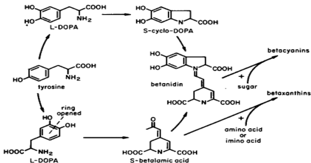
Figure 3. The main structure of betalain
