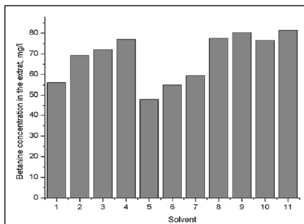
Figure 6. Betanine concentration in primary extracts
